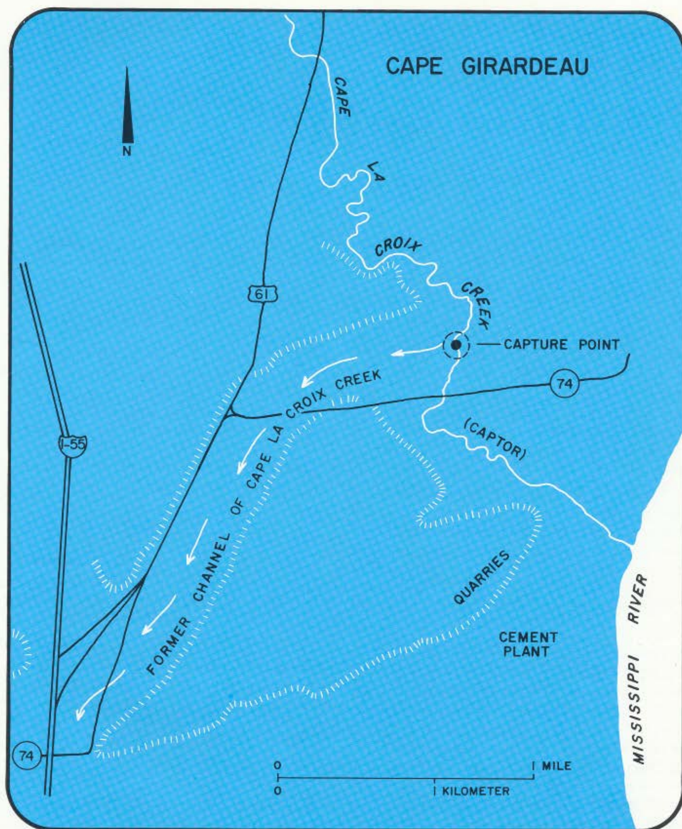
Figure 80 Stream capture at south edge of Cape Girardeau.
