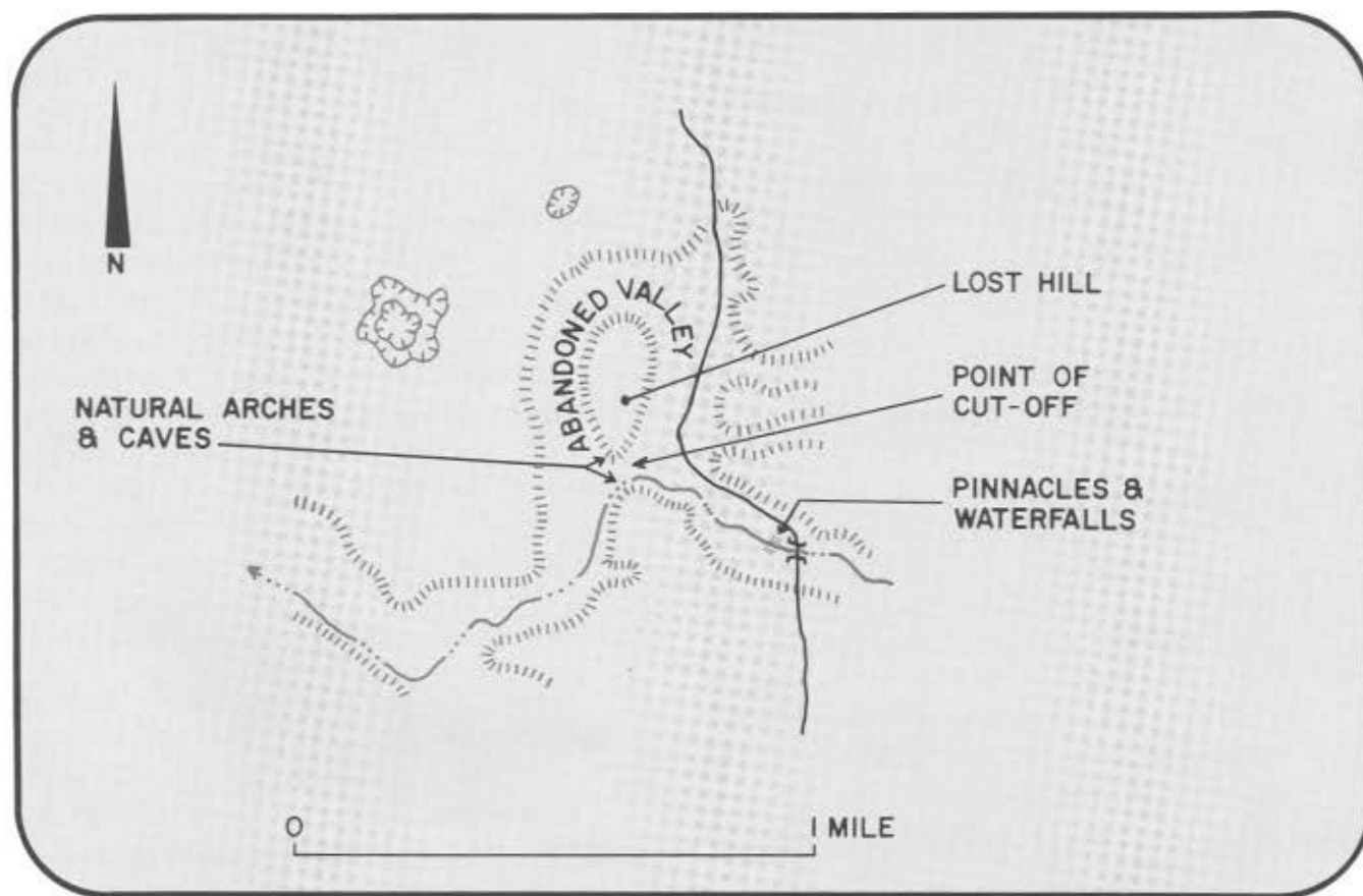
Figure 140 Dry Sac Lost Hill Area near Springfield.
