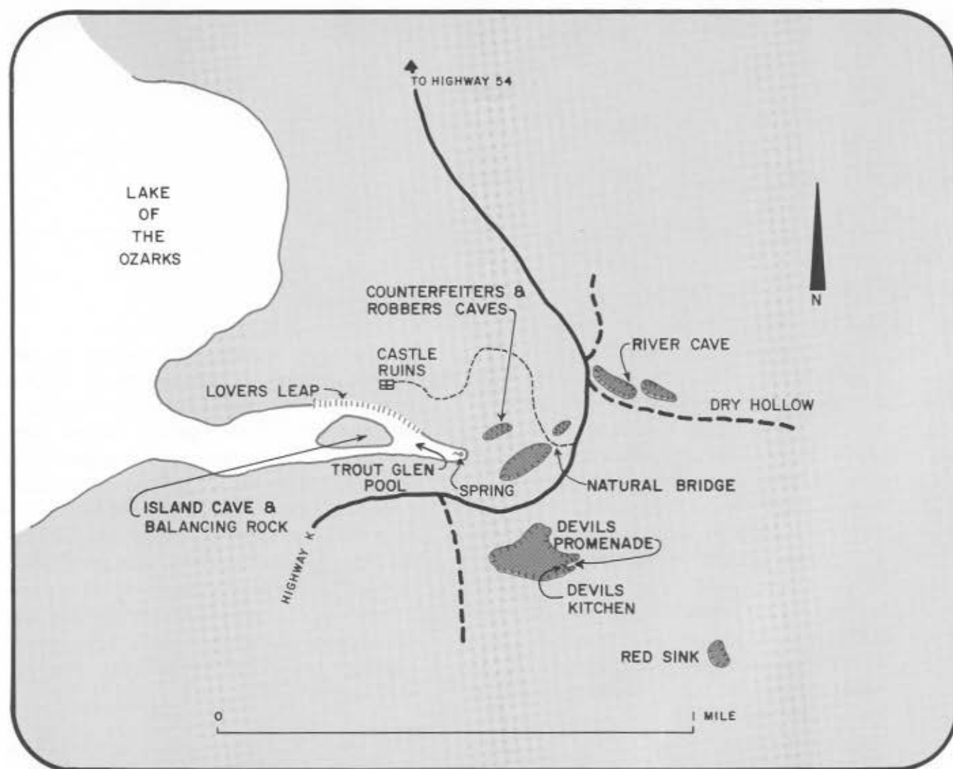
Figure 138 Hahatonka area, Camden County.
