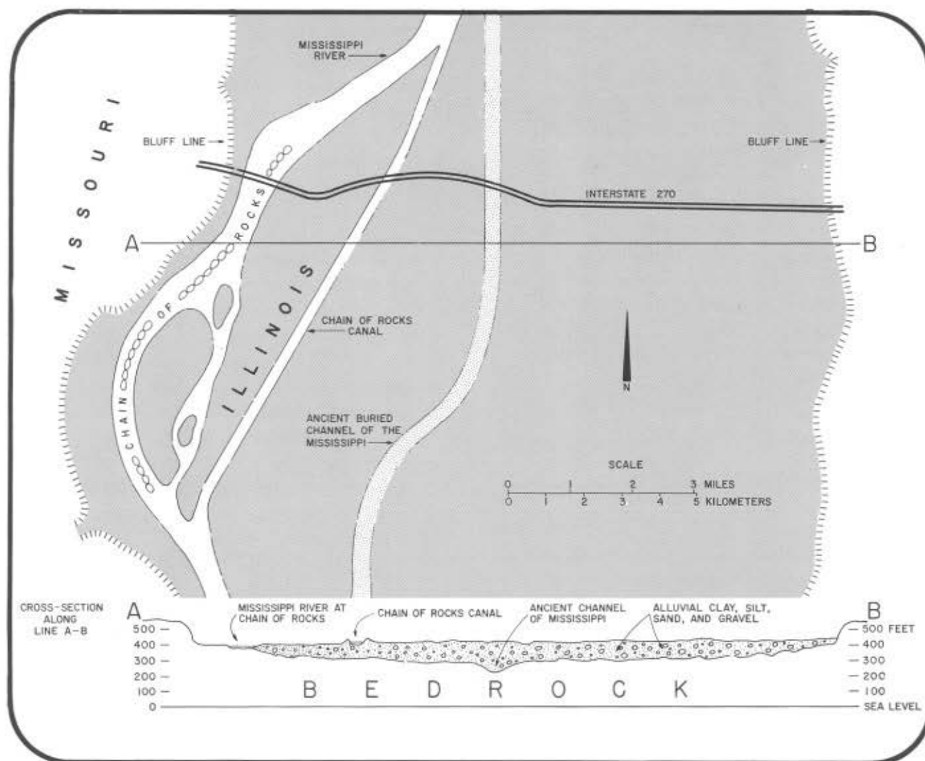
Figure 30 Channel-bedrock relationships in Chain-of-Rocks (St. Louis) area.
