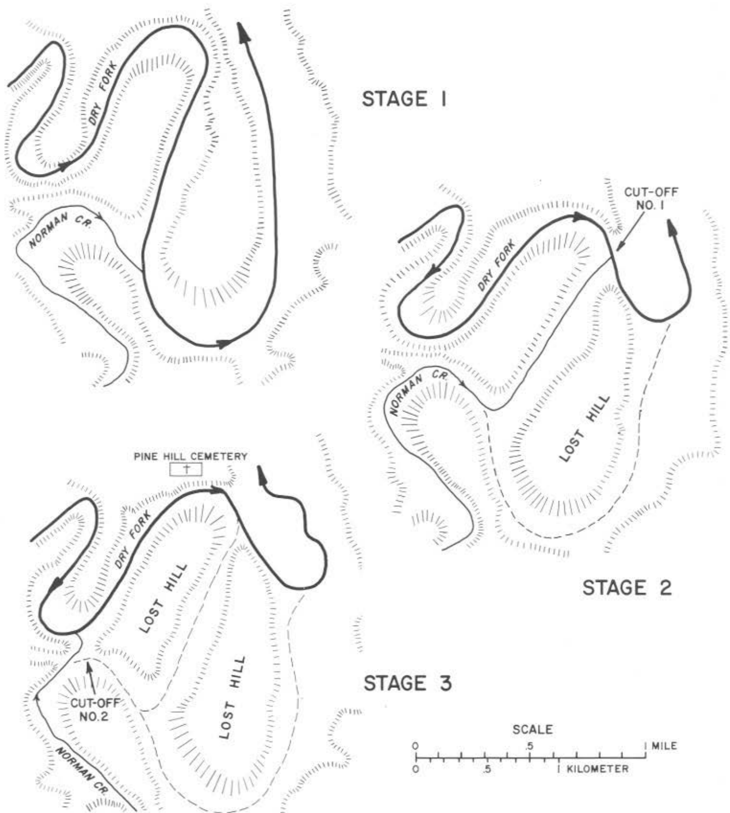
Figure 71 Postulated sequence of cutoffs that created double lost hills (No. 166) on Dry Fork in Phelps County.
