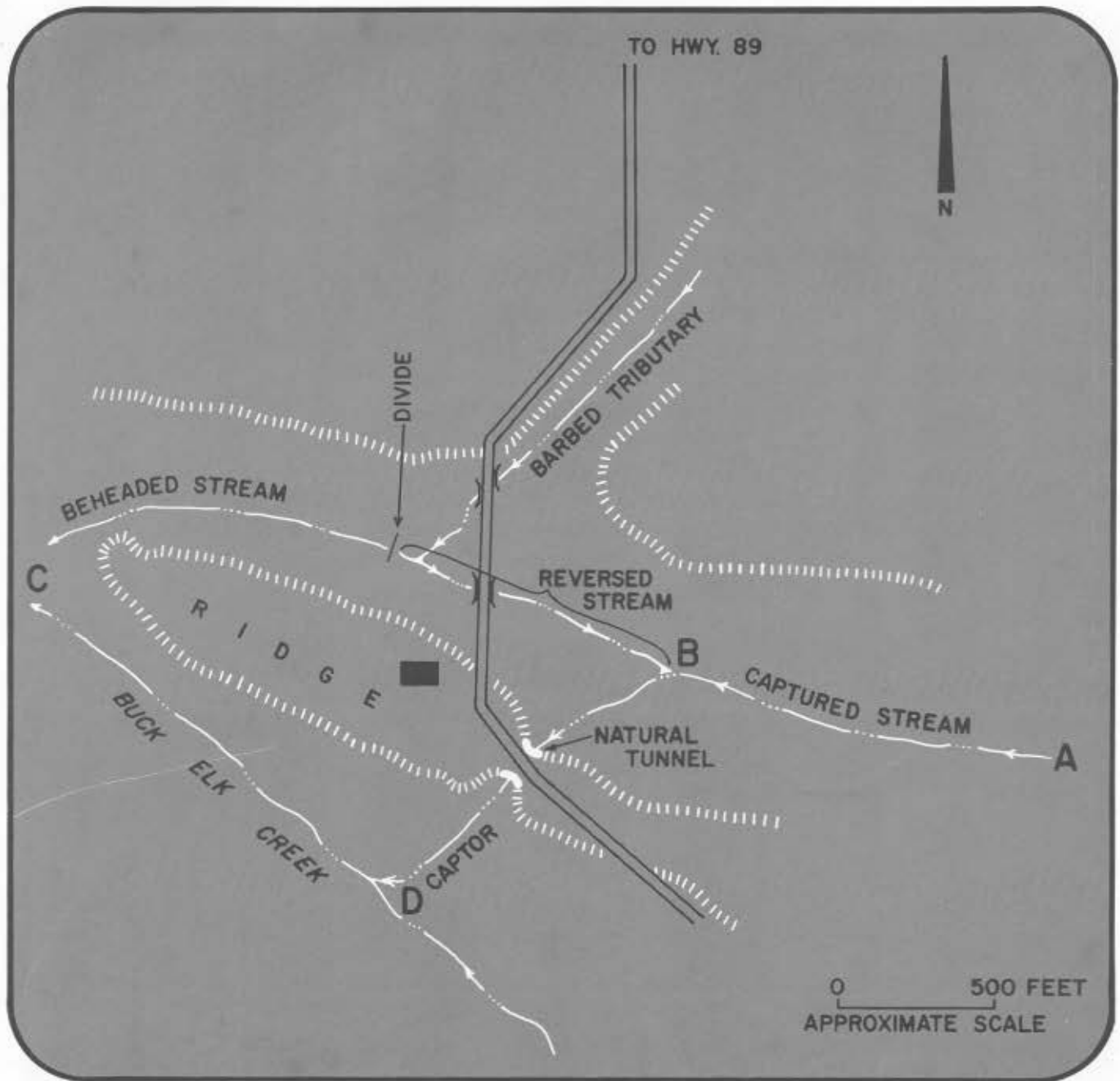
Figure 130 Tunnel Cave Natural Tunnel and stream piracy.
