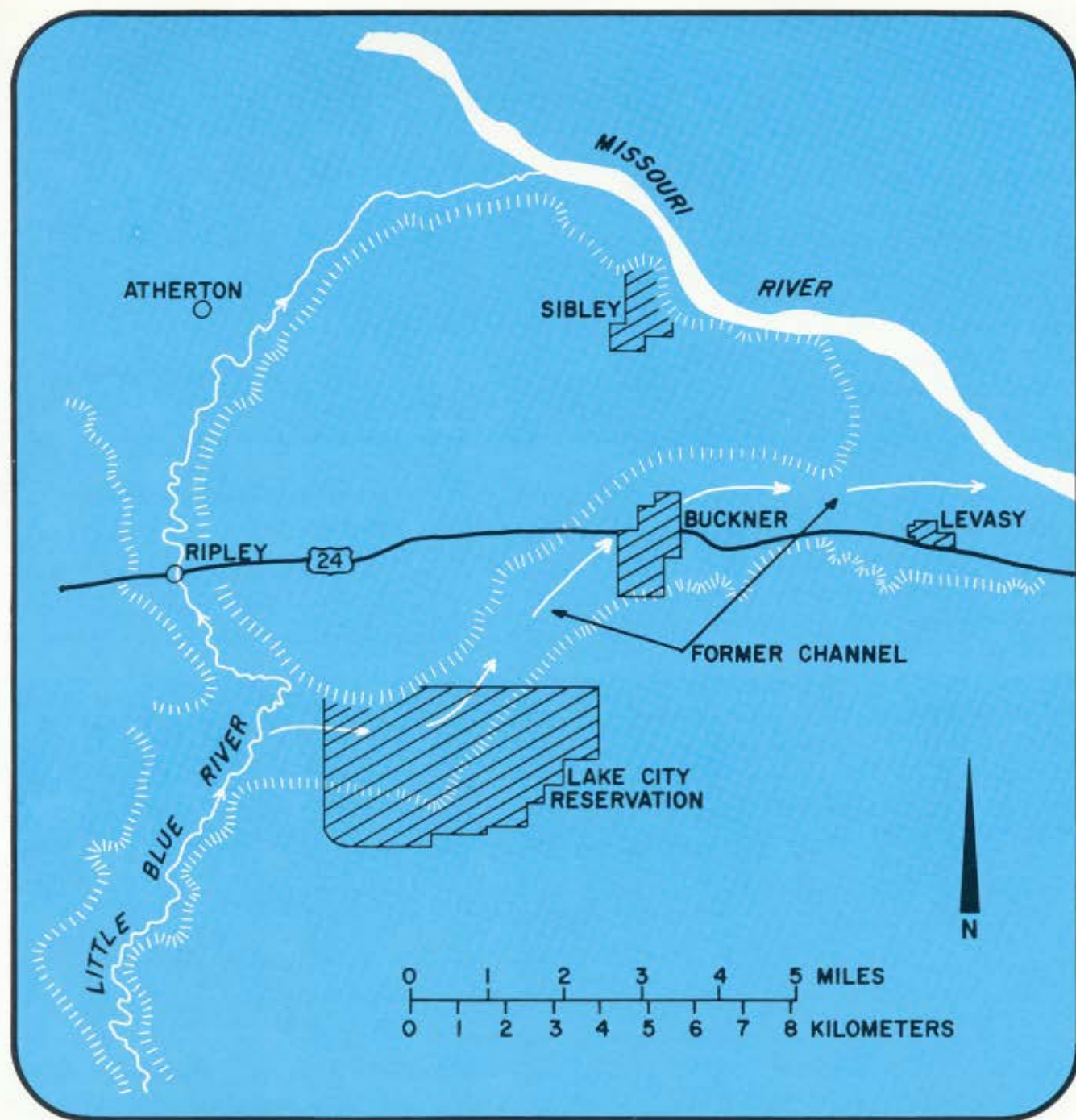
Figure 81 Lake City piracy.
