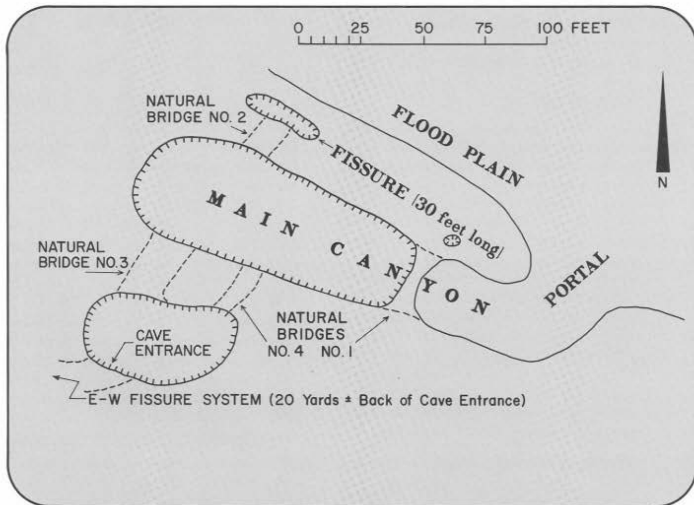
Figure 141 Kassel Cave Natural Bridges.
