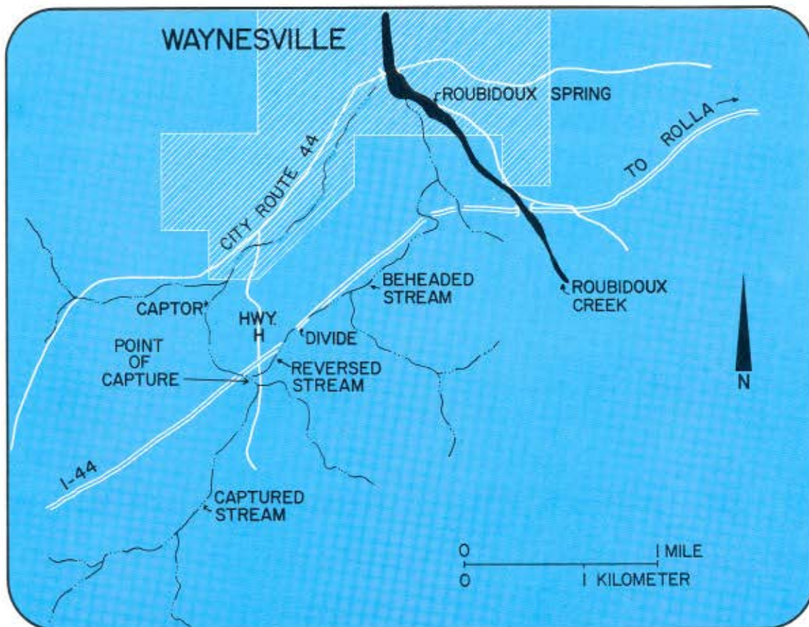
Figure 82 Waynesville stream capture.
