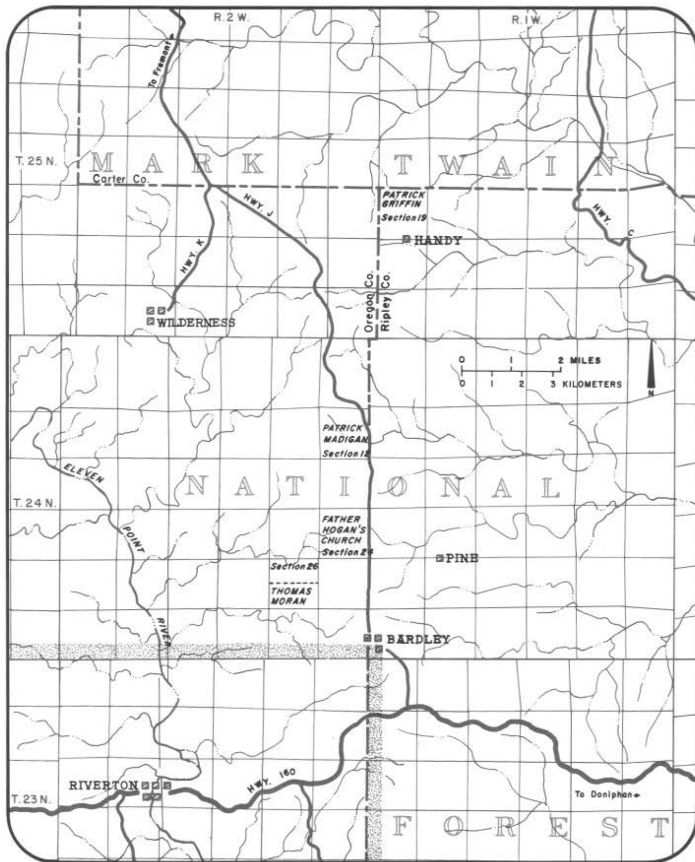
Figure 154 The Irish Wilderness
