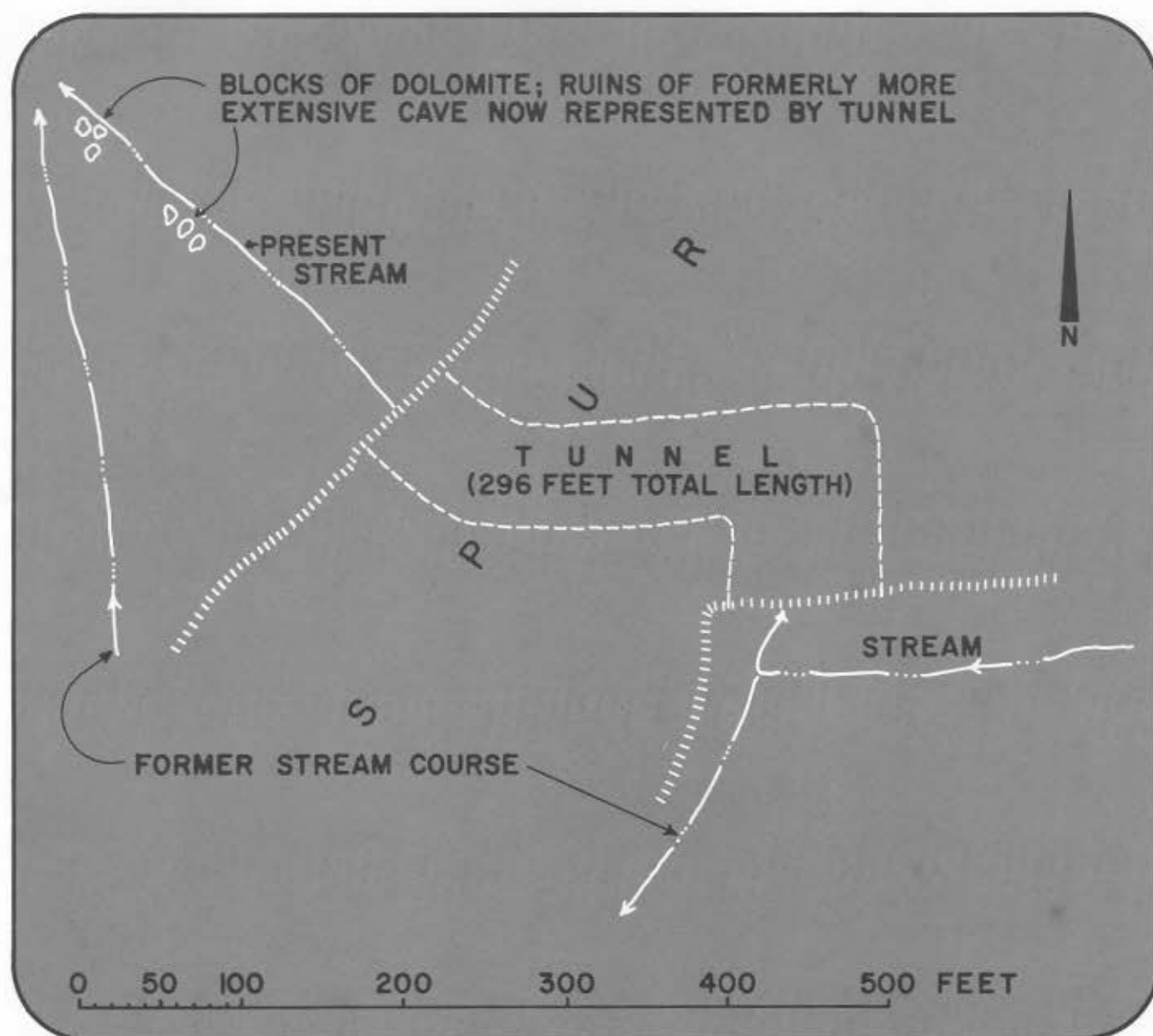
Figure 132 Subterranean piracy and Bennett Spring Natural Tunnel.
