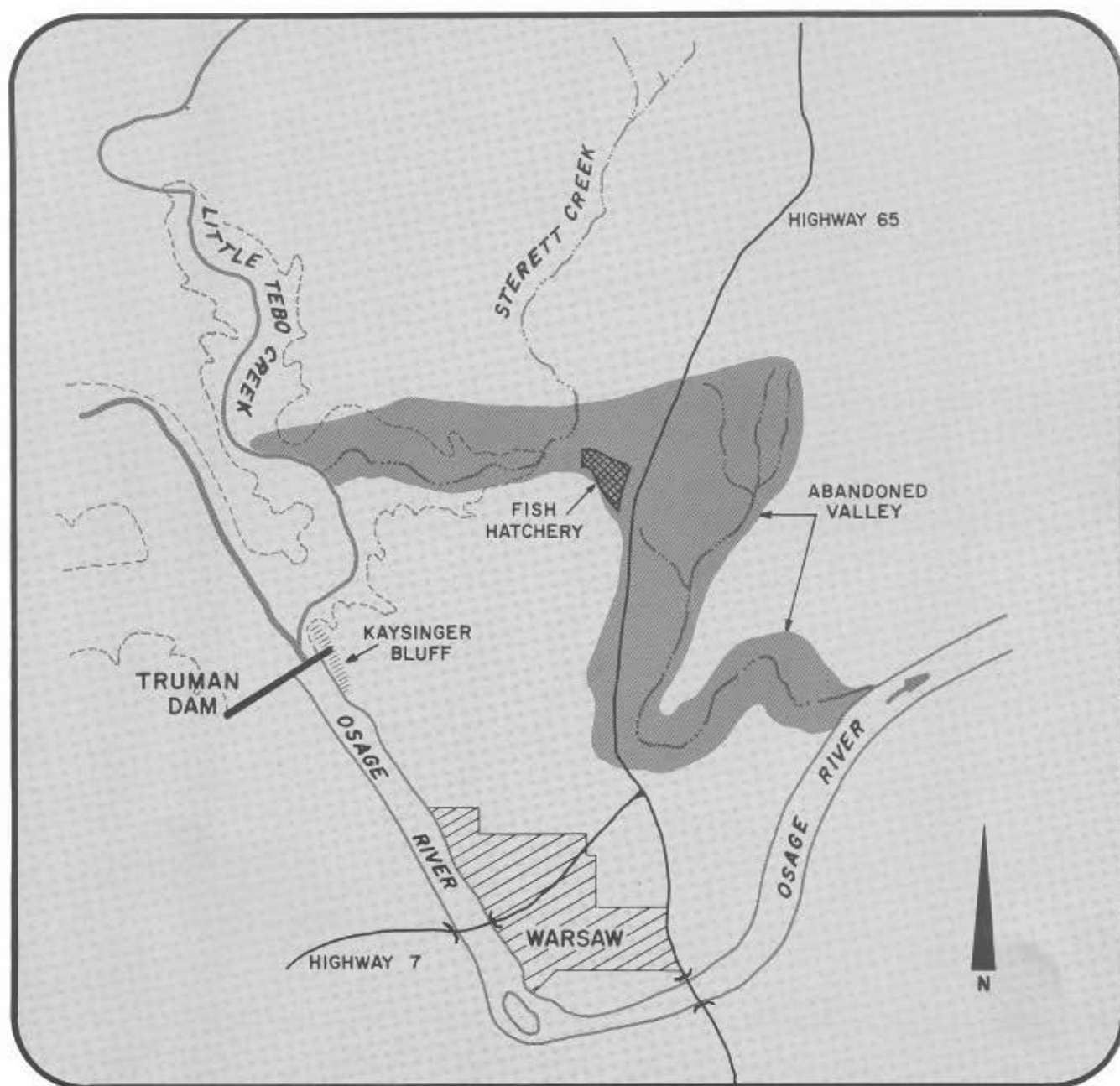
Figure 78 Little Tebo Creek capture at Warsaw.
