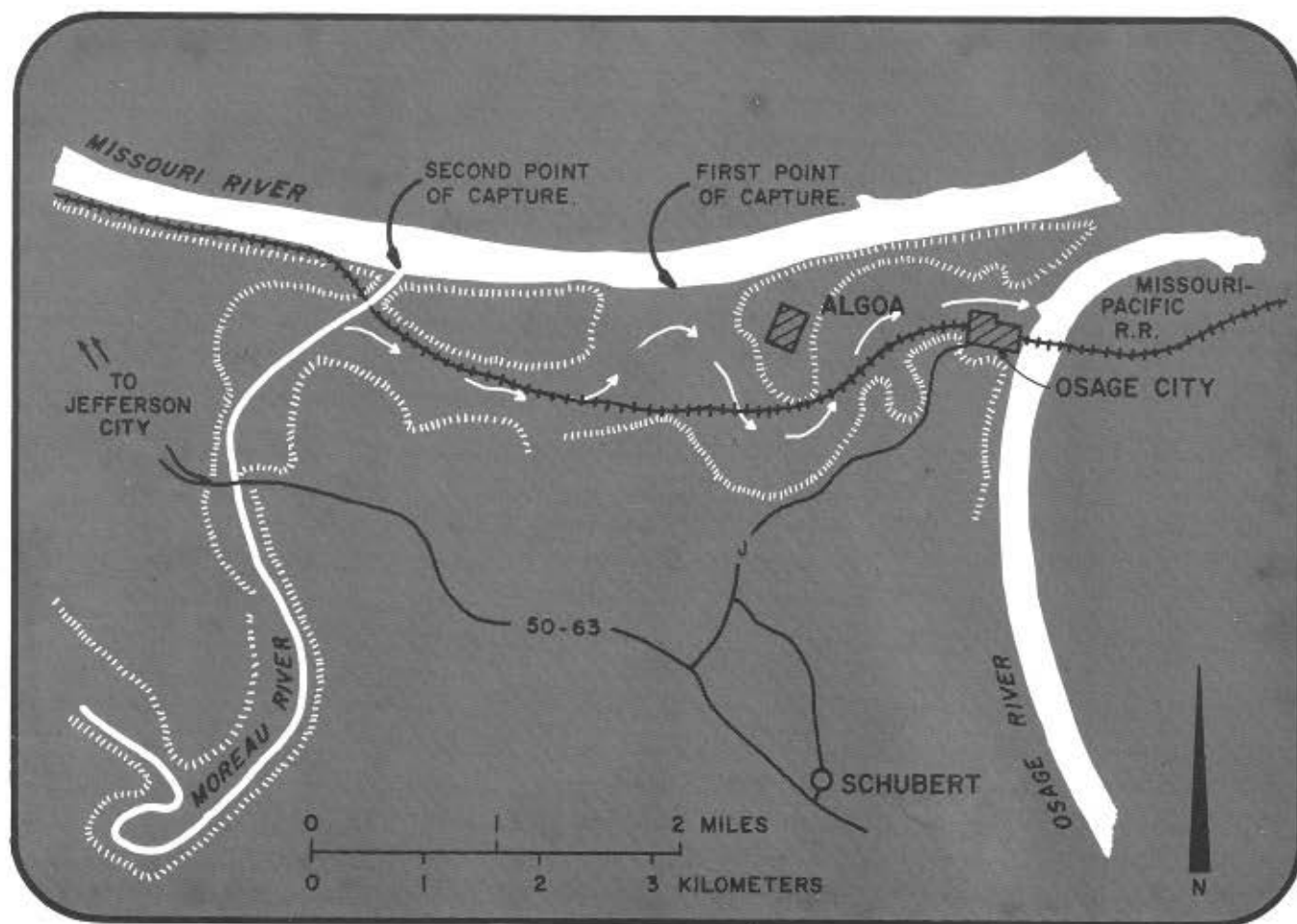
Figure 79 Moreau River capture east of Jefferson City.
