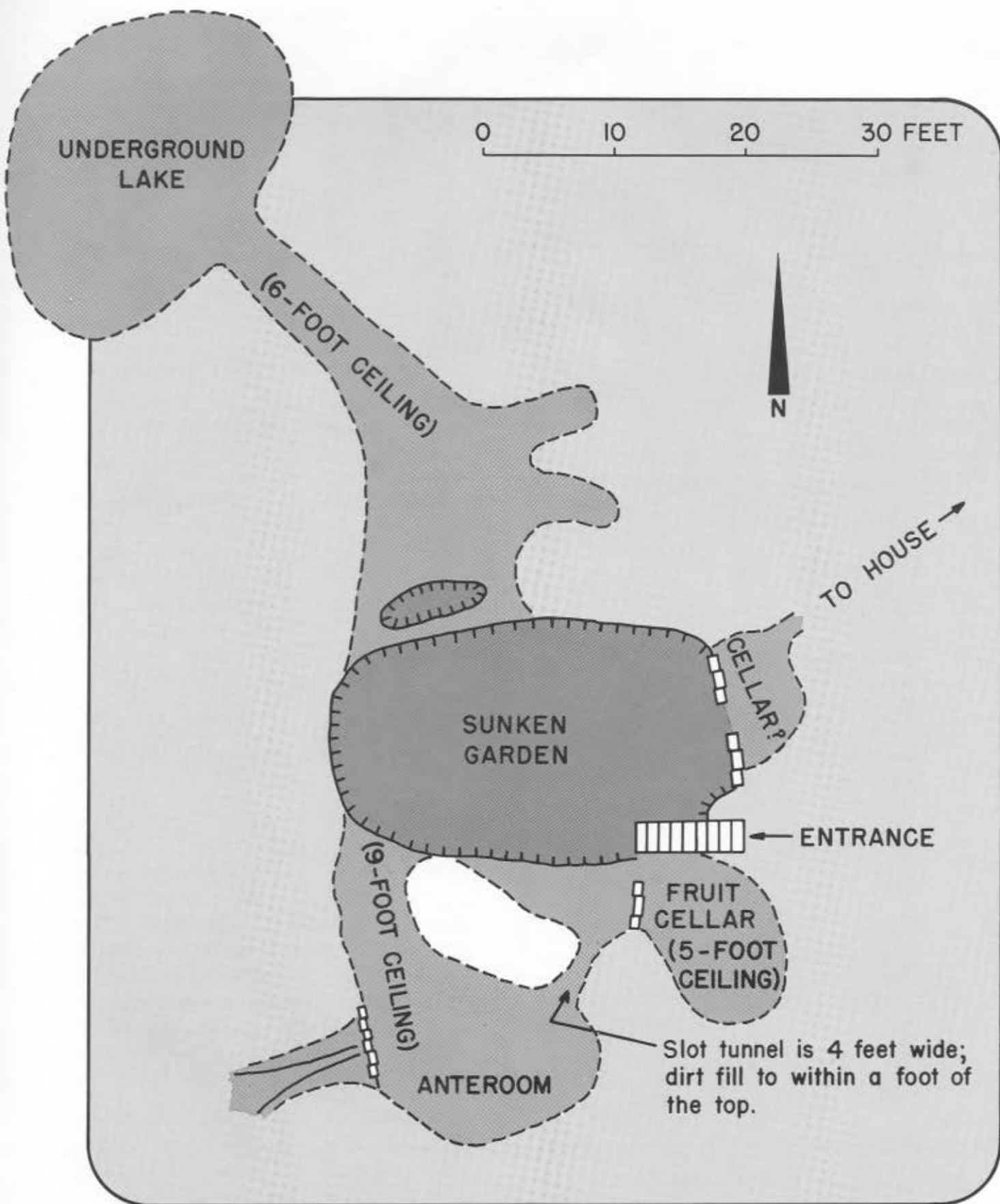
Figure 142 Ratcliff Cave Sunken Garden.
