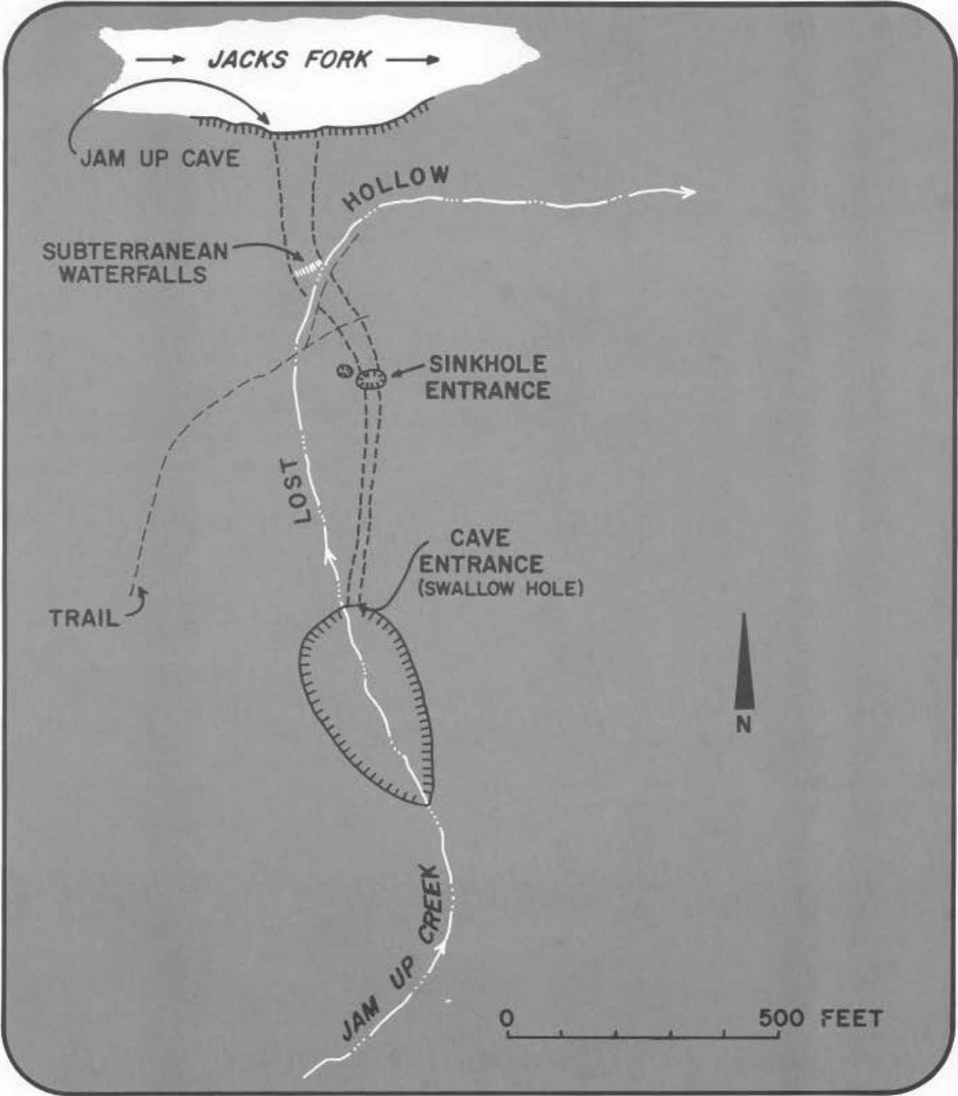
Figure 129 Sketch map of Jam Up Natural Tunnel System.
