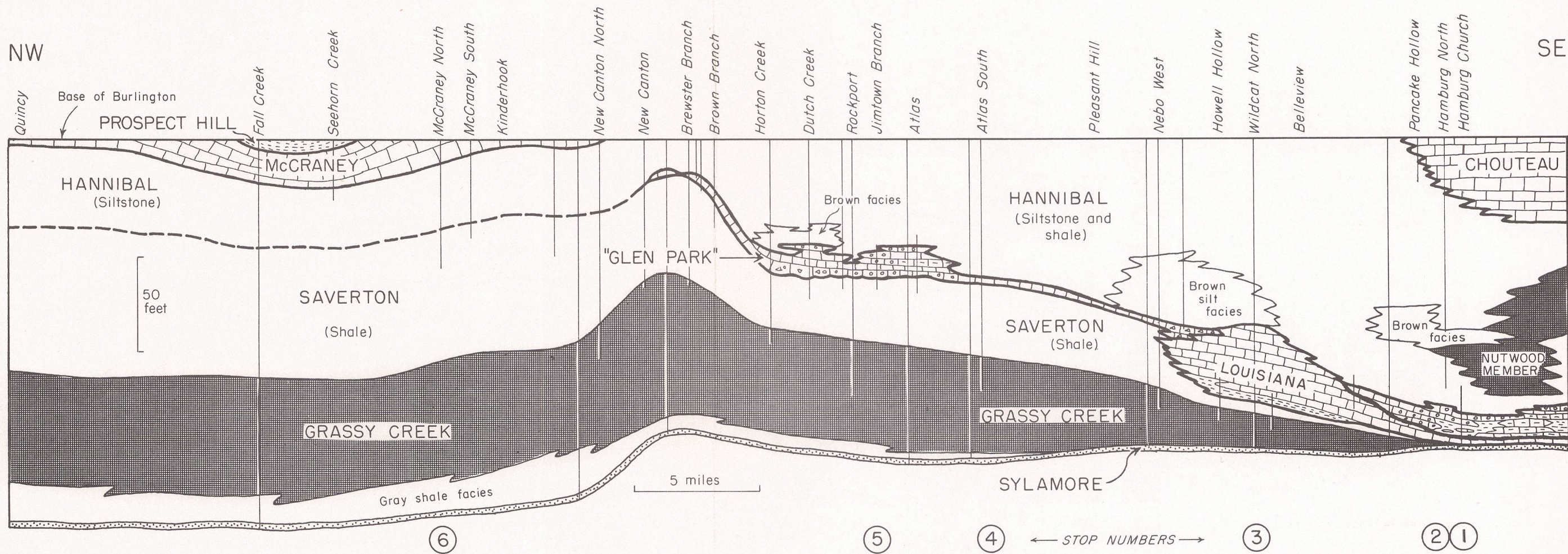
Fig. 3. Generalized Cross Section of Upper Devonian — Kinderhookian Series in Bluffs of Mississippi River.
