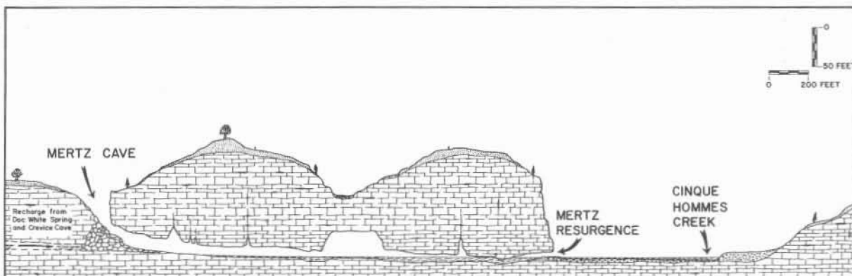
Figure 20 -- Diagrammatic longitudinal section of the lower part of Mertz Cave and Mertz Resurgence.
