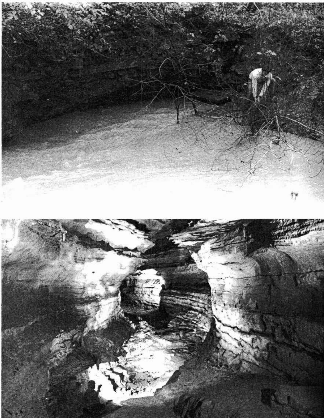
Figure 12 -- Blue Spring (12A), shown after heavy rainfall, is the largest perennial spring along Blue Spring Branch. The Moore Cave System (12B) is part of the conduit system that transports water to the spring.
