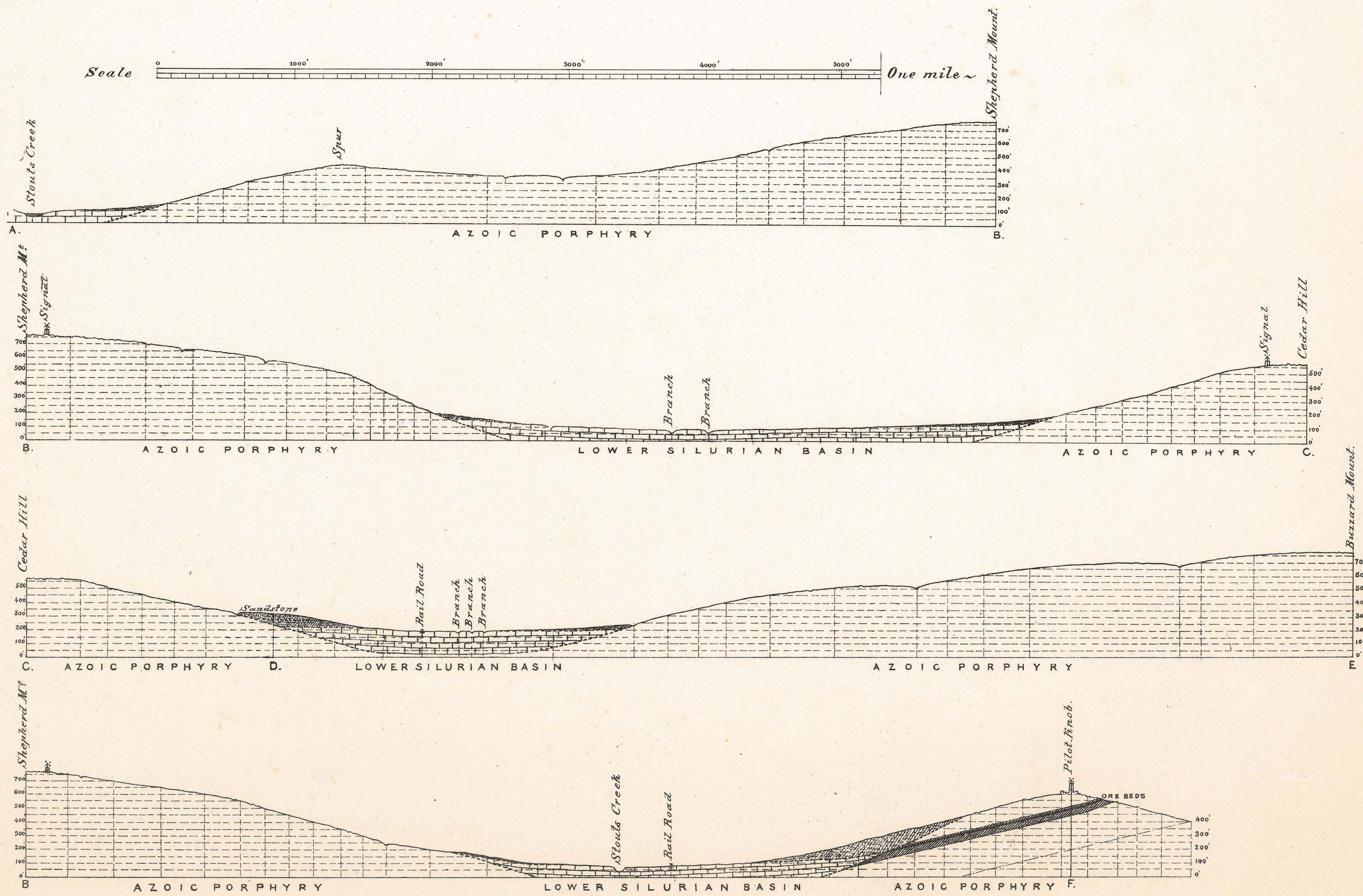
TOPOGRAPHICAL SECTIONS OF THE PILOT-KNOB DISTRICT REFERRING TO PLATE I.
