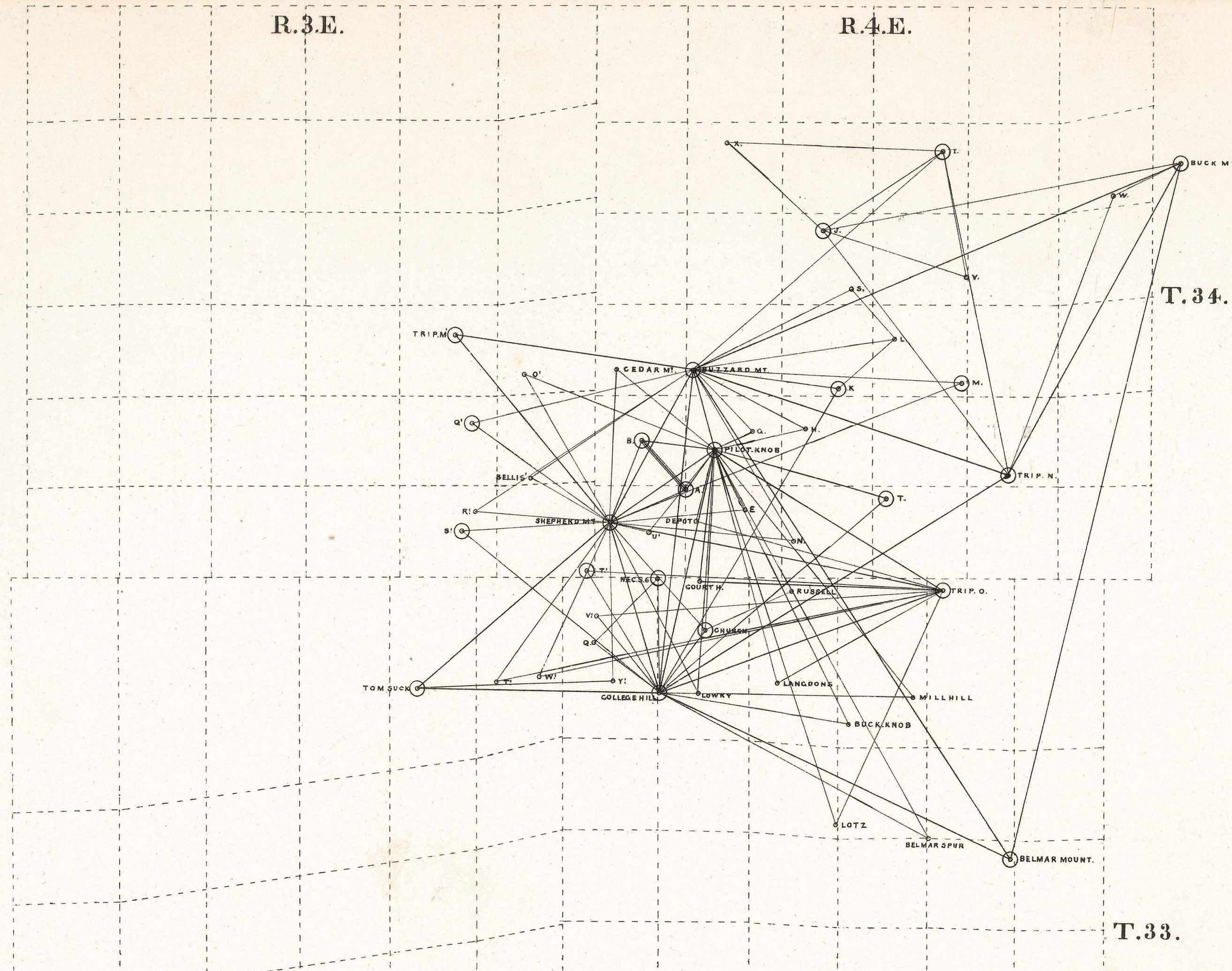
DIAGRAM SHOWING THE POINTS ESTABLISHED BY TRIANGULATION IN THE PILOT-KNOB DISTRICT IN 1872.
