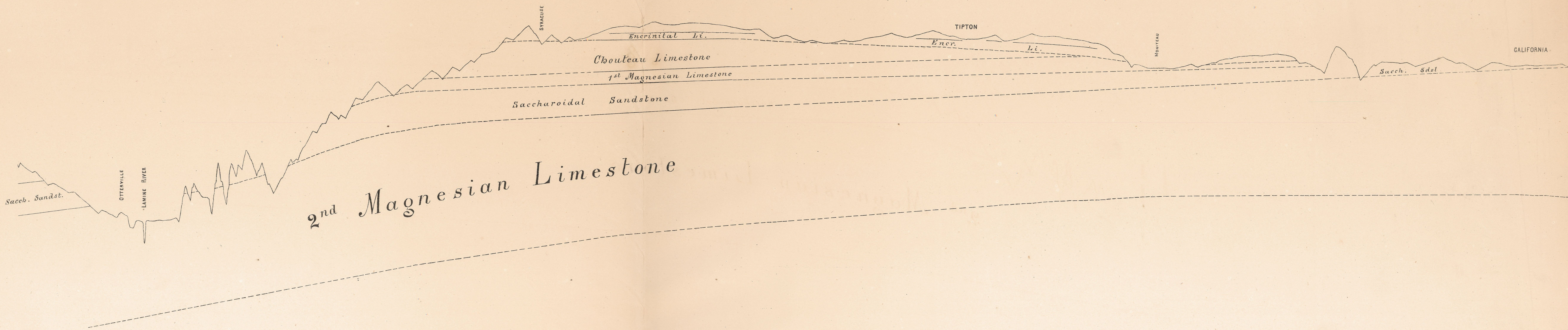
PROFILE SHOWING RELATION OF SURFACE TO ENCHRINITAL LIMESTONE ON THE TRUE SCALES.
