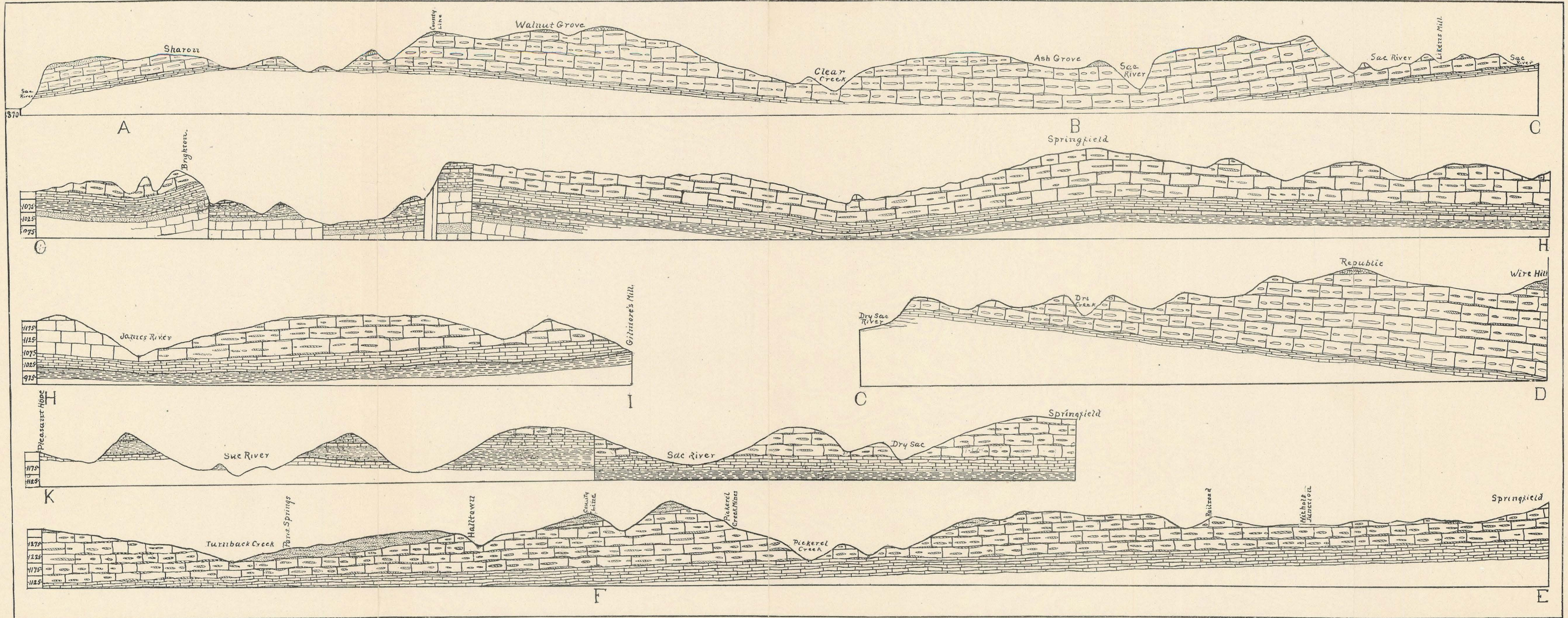
Structure Sections, Springfield Sheet.
