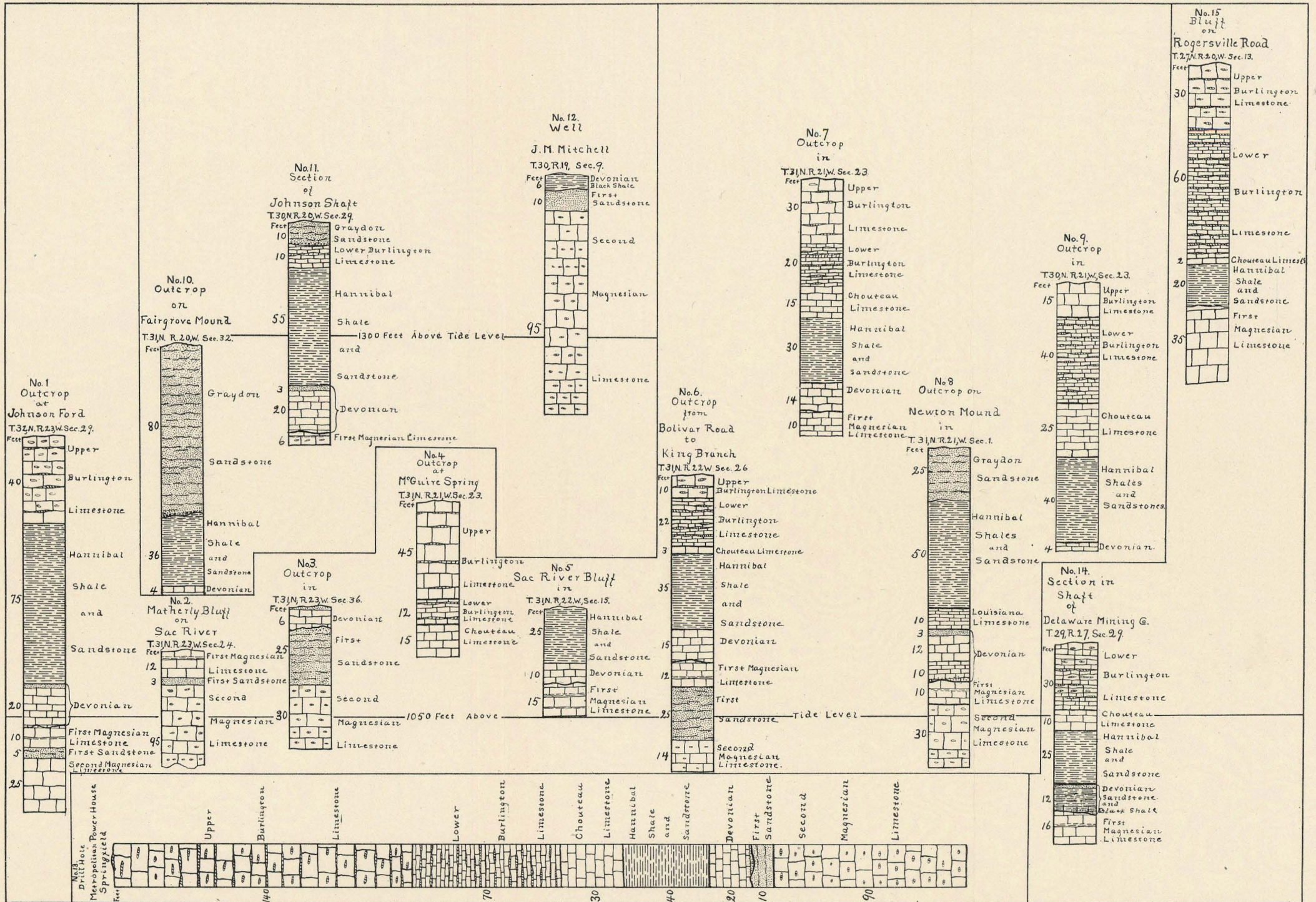
Columnar Sections, Springfield Sheet.
