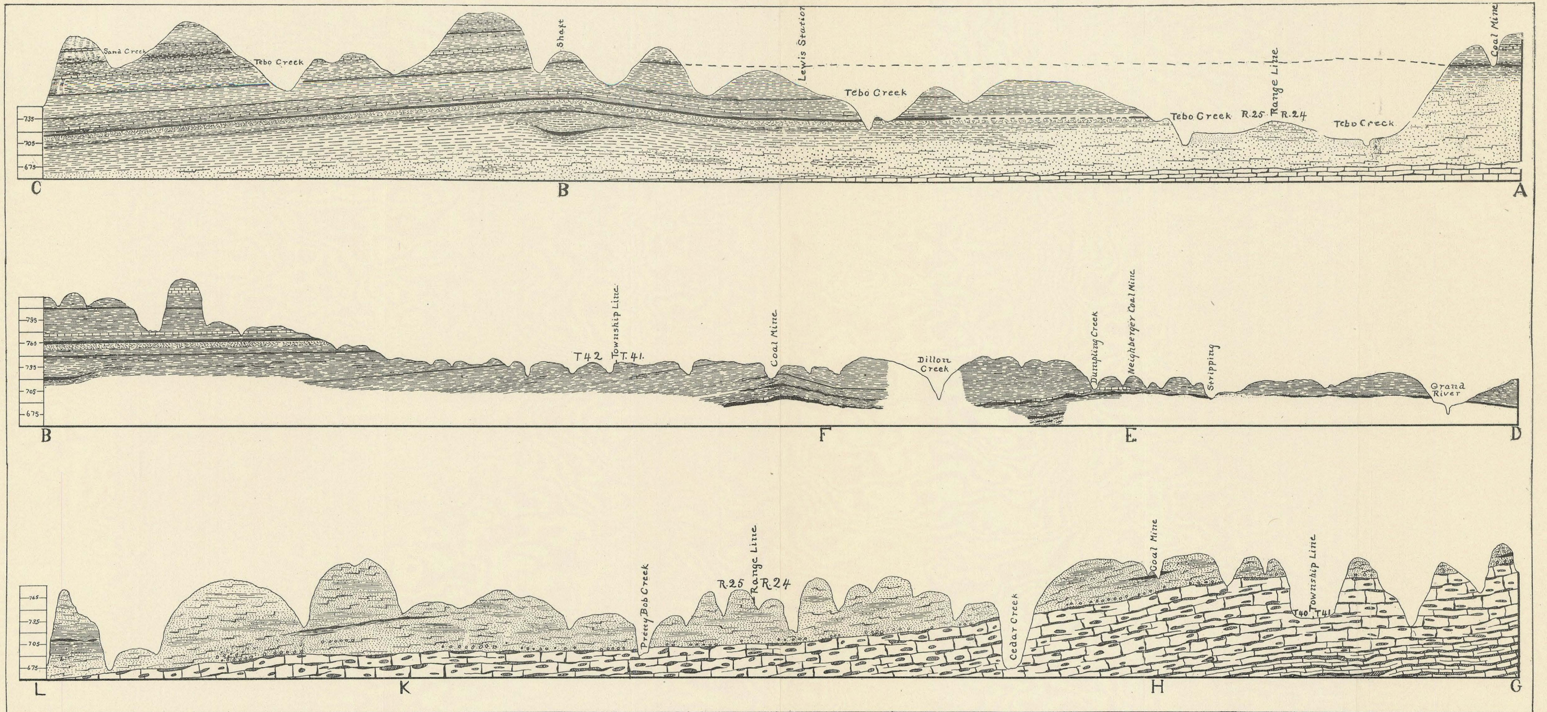
Geological Cross Sections, Calhoun Quadrangle.
